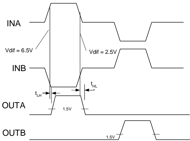
Figure 3 ARINC 429 Input to Logic Output Switching Waveform
