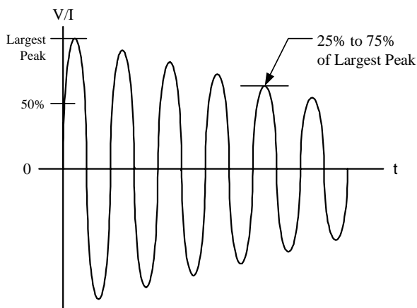
Figure 5 DO160 Lightning Induced Transient Voltage Waveform #3.
