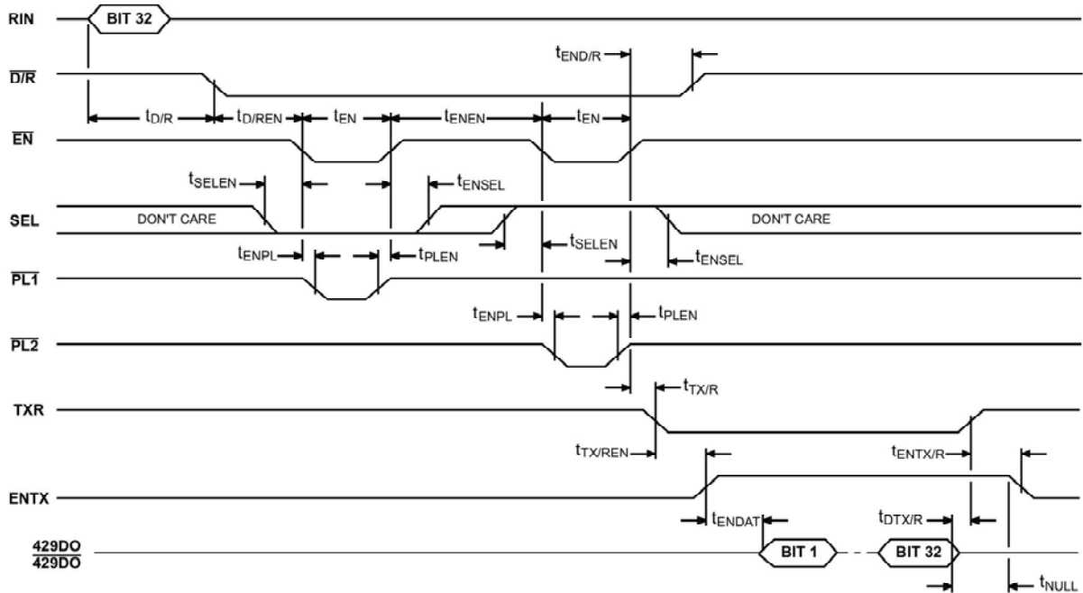
Figure 12 Repeater Operation
