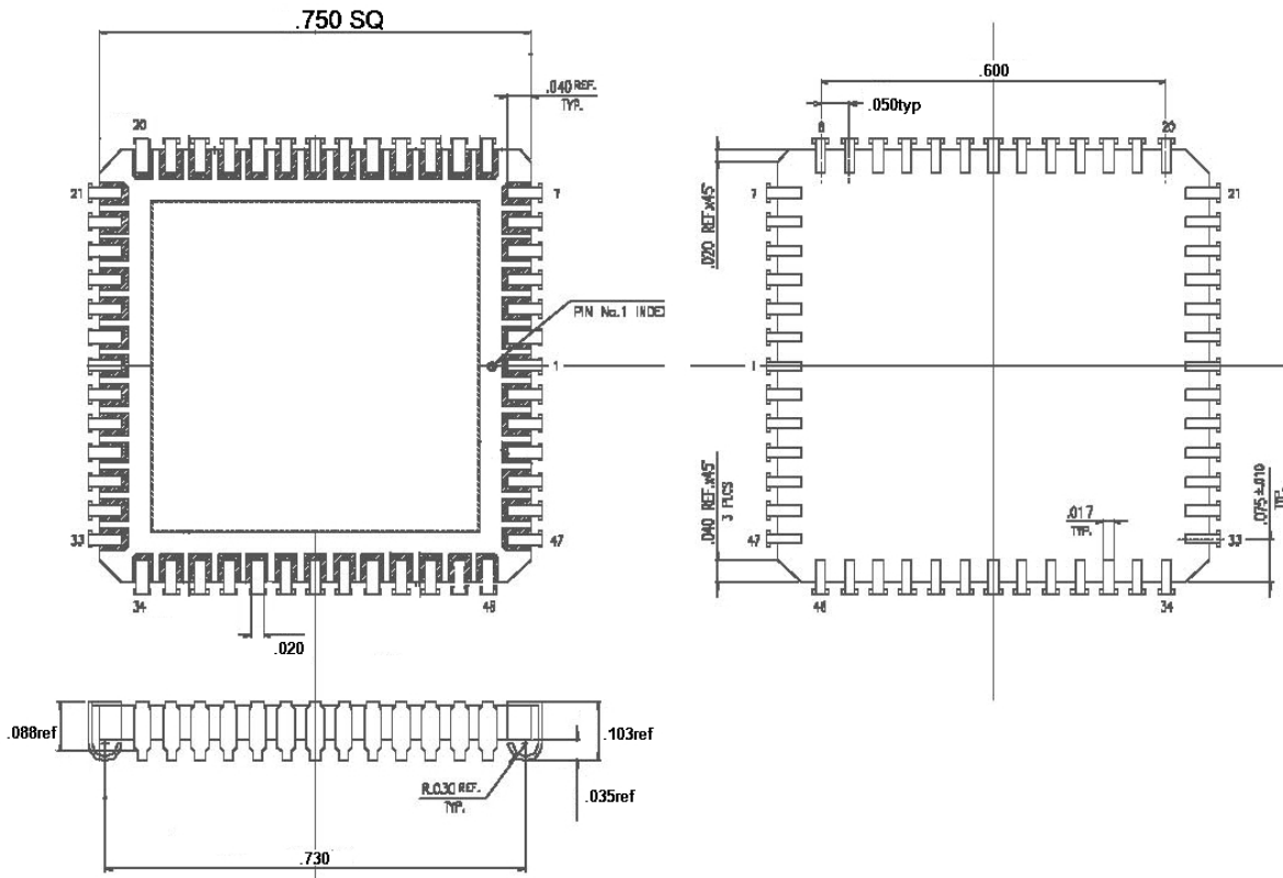
Figure 14 52L CQFJ
