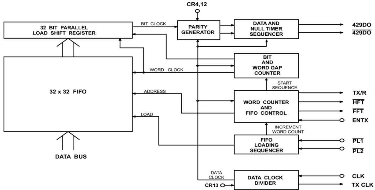
Figure 2 Transmitter Function Diagram
