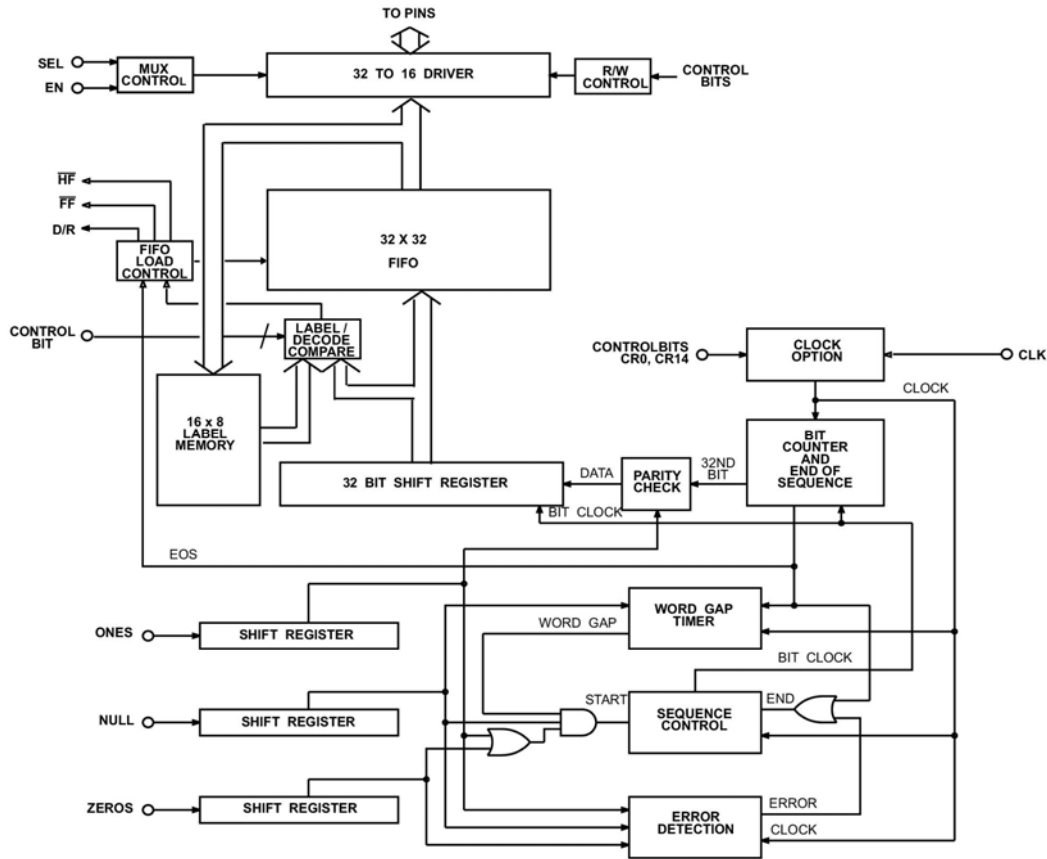
Figure 1 Receiver Function Diagram
