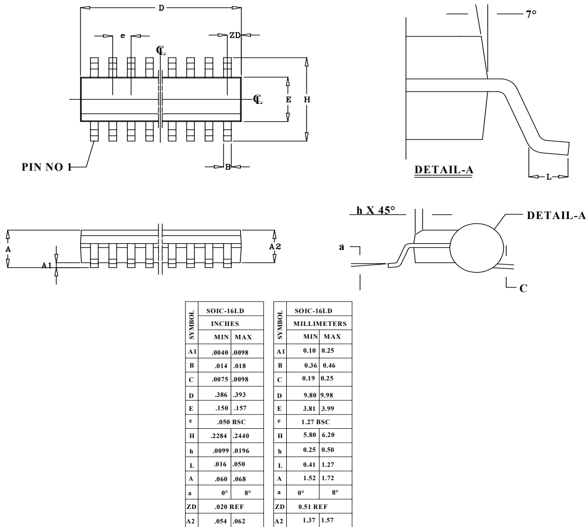
Figure 8 16 Lead Narrow Body SOIC Outline Drawing
