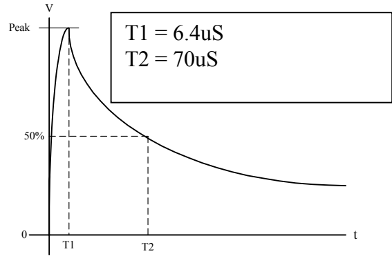
Figure 5 Voltage Waveform 4
