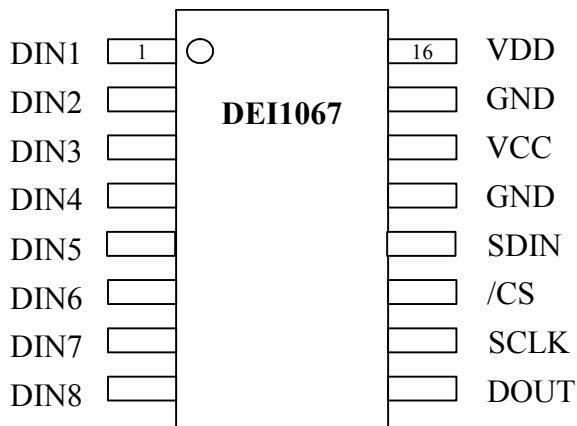
Figure 1 DEI1067 Pin Assignment (16 Lead NB SOIC)
