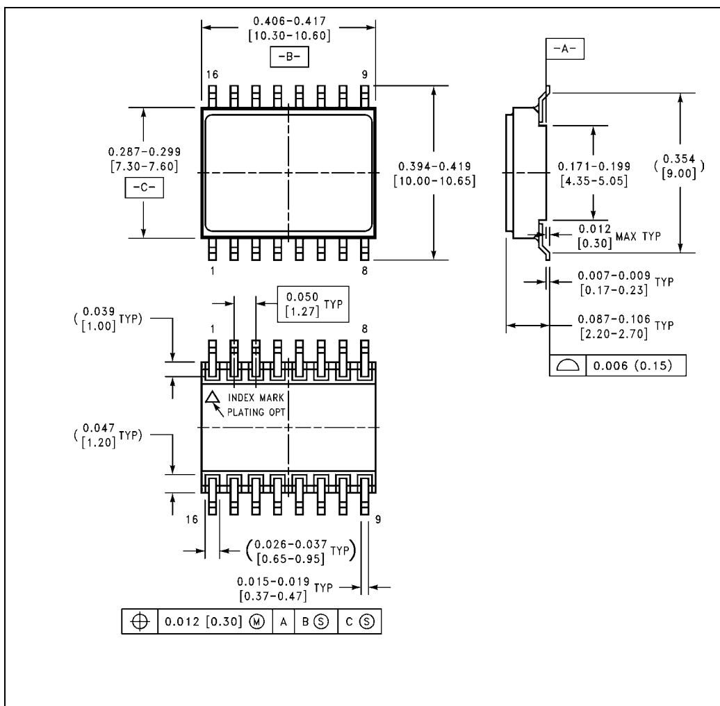
Figure 12 16 Lead CSOP Outline Drawing
