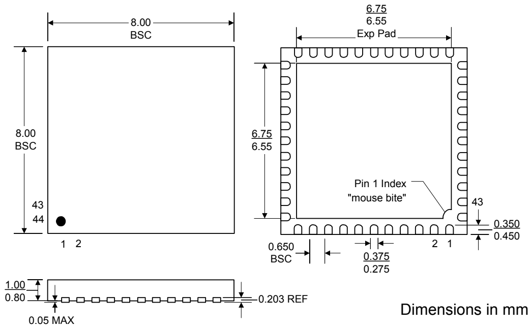
Figure 18: 44 Lead 8X8 MLPQ Mechanical Outline (44 MLPQ)
