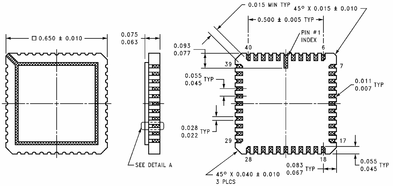
Figure 17: 44 Lead CLCC Mechanical Outline (44 CLCC)
